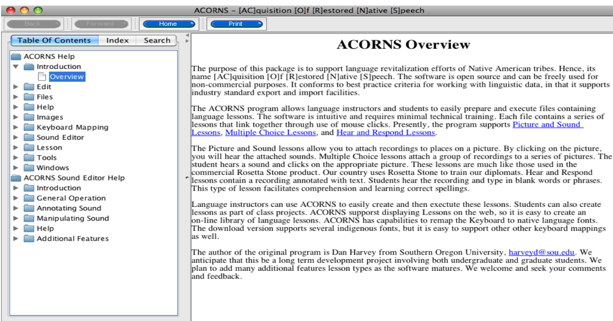
Figure 5-2 Help command
