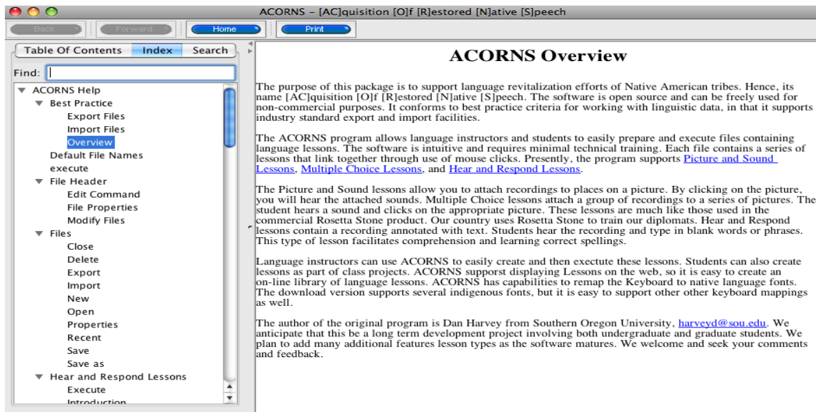
Figure 5-3 Index mode
