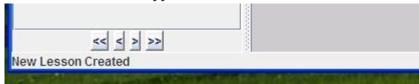
Figure 5-1 Feedback message
