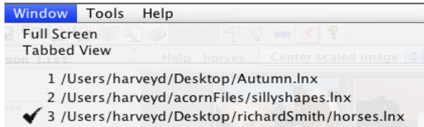
Figure 2- 9 Windows commands
