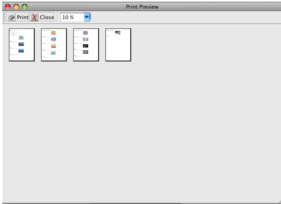
Figure 2- 12 Print Preview
