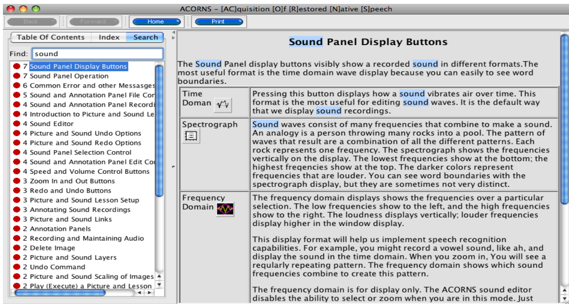
Figure 5-4 Search mode
